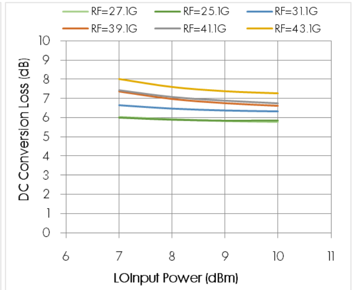
Conversion Loss vs. LO Power
