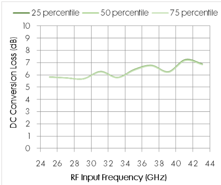
Conversion Loss vs. Frequency
