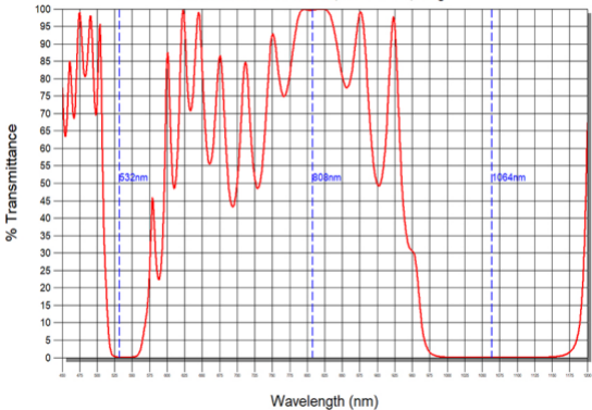
Dual HR 1064nm and 532nm, Pass 808nm, 0deg
