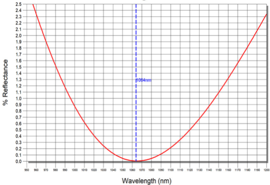
A1500: MAXCOAT AR @ 1064nm on Nd:YAG
