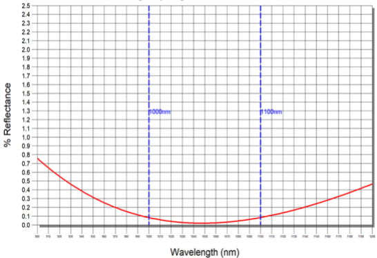
A1142: Single Layer MgF2 on TGG for 1000 - 1100nm
